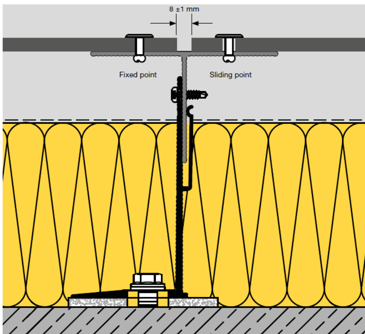
Figure 1.0 – Vertical and Horizontal Panel Joints
