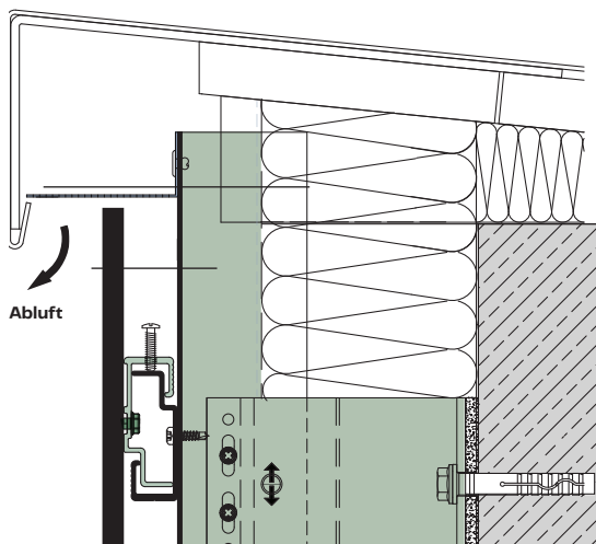
Attika A109
