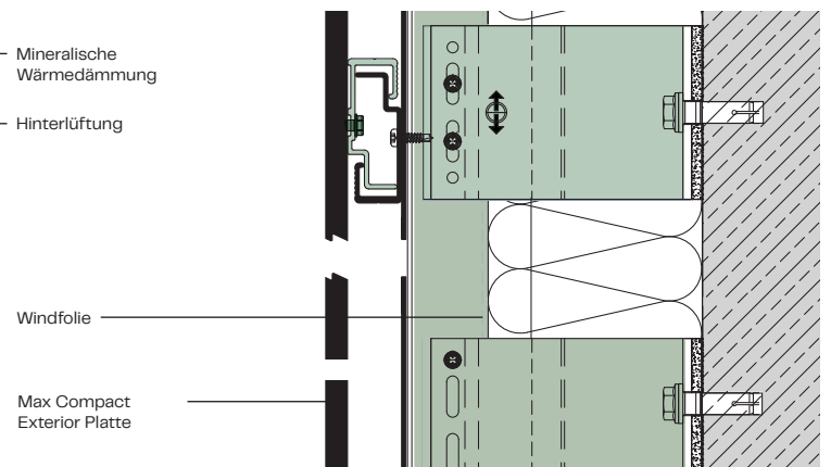
Horizontalfuge A110
